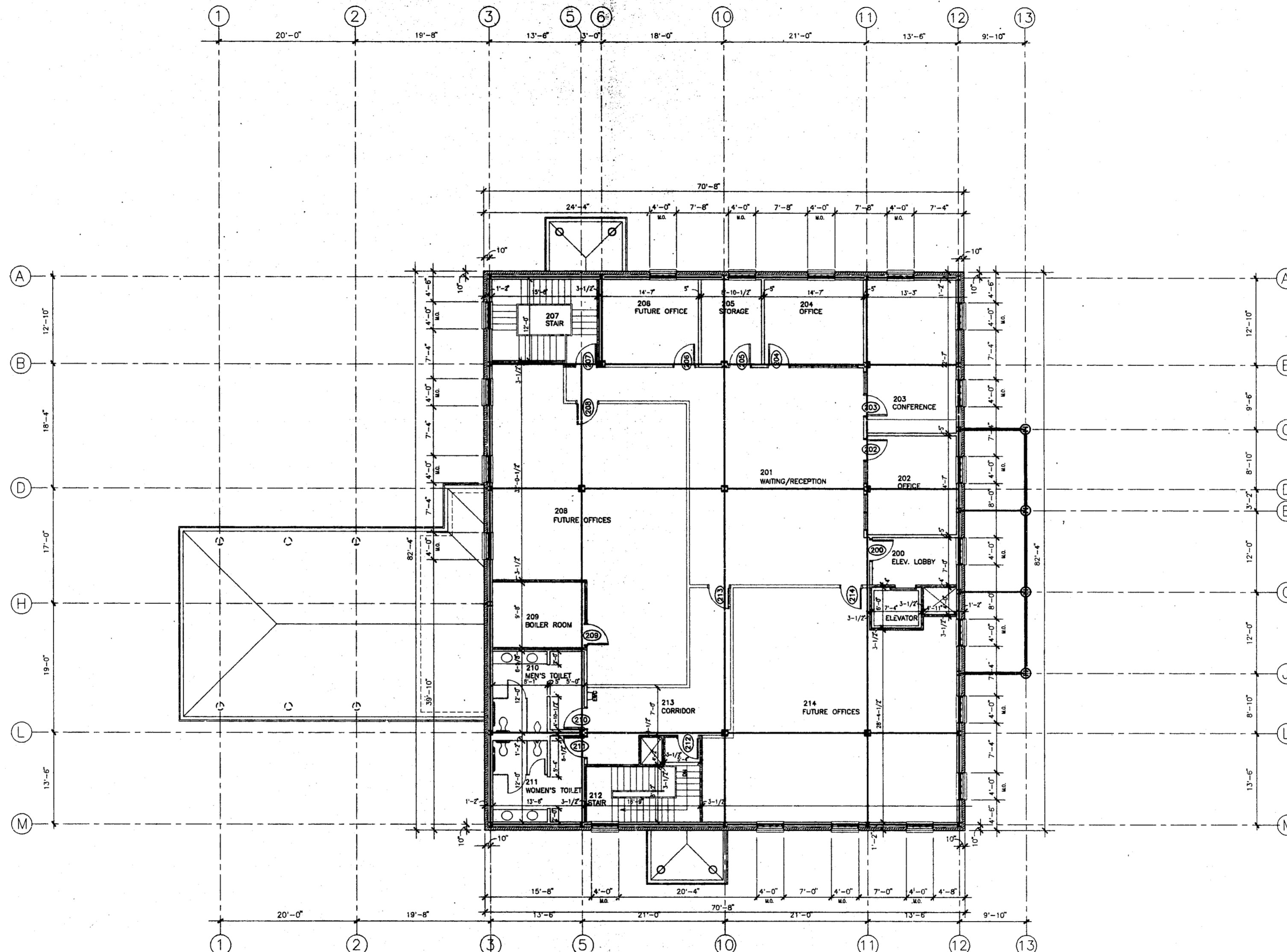
A2.01 SECOND FLOOR PLAN SCALE: 1/8" = 1'-0"
