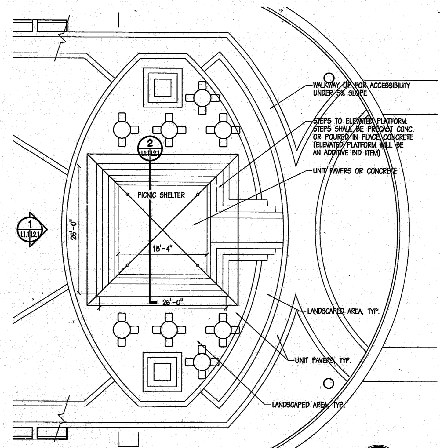
3 ENLARGED PICNIC SHELTER PLAN SCALE: 1/8"=1'-0"
