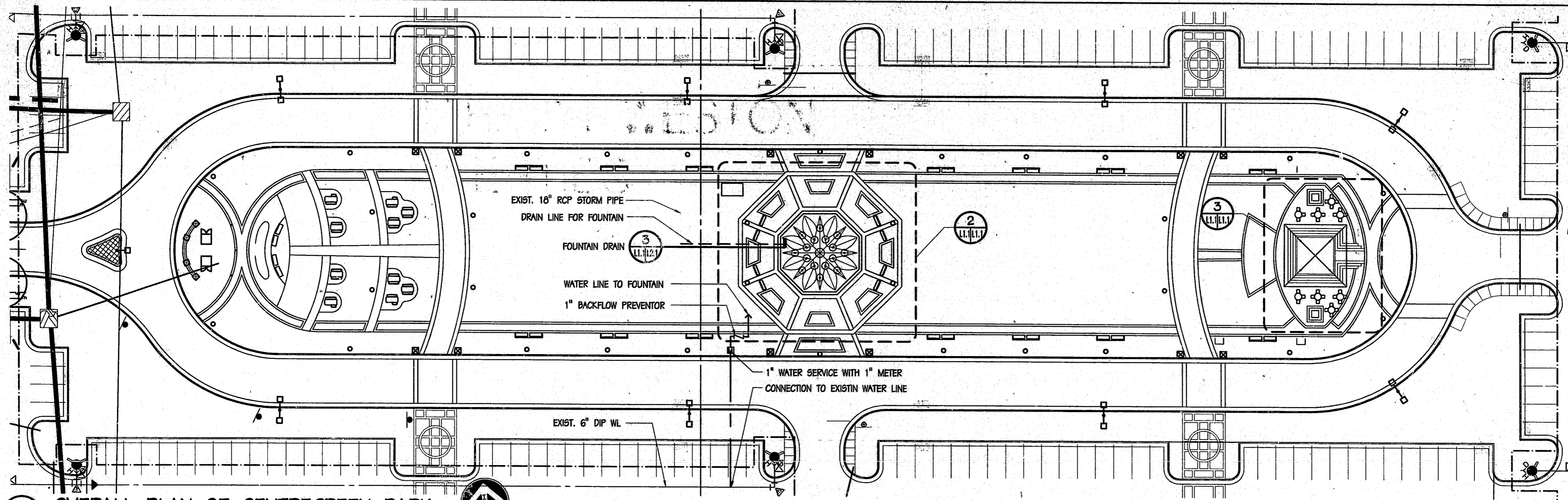
1 OVERALL PLAN OF CENTREGREEN PARK SCALE: 1"=25'-0"
