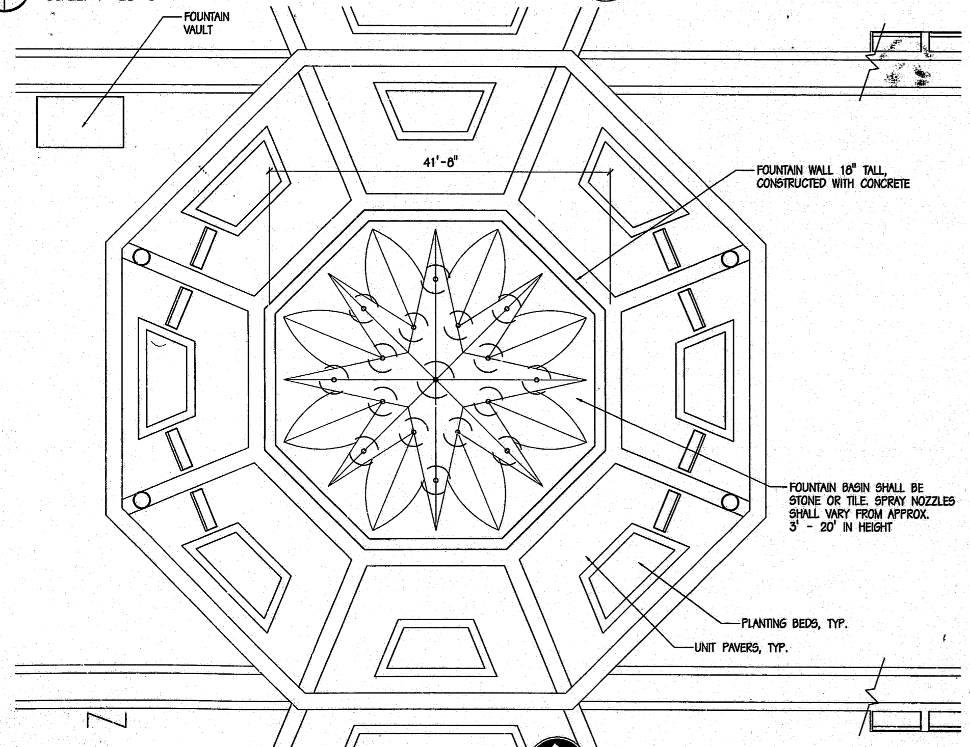
2 ENLARGED FOUNTAIN PLAN SCALE: 1/8"=1'-0"
