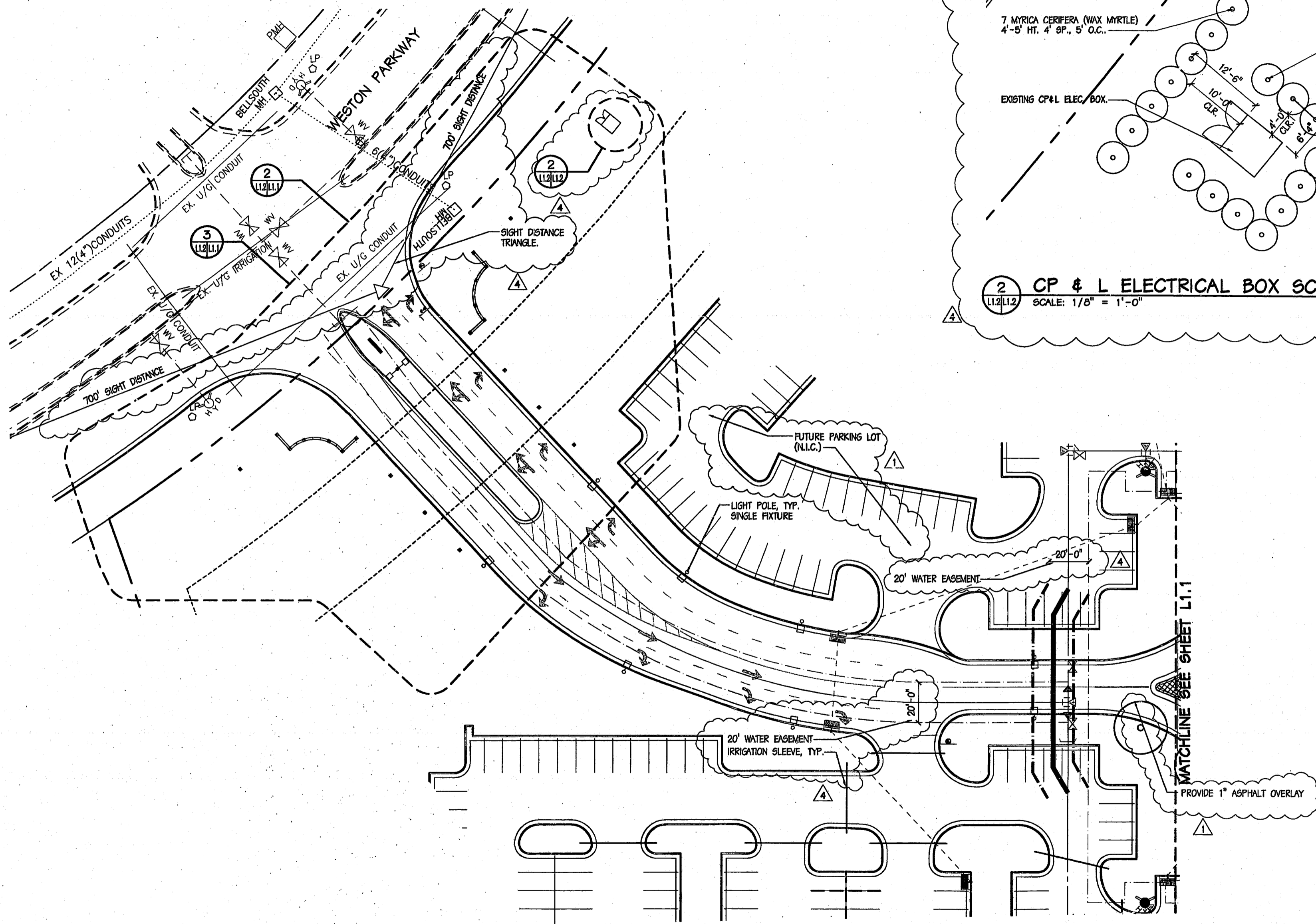
1 HARDSCAPE PLAN OF CENTREGREEN L1.2/L1.2 SCALE: 1" = 25'
