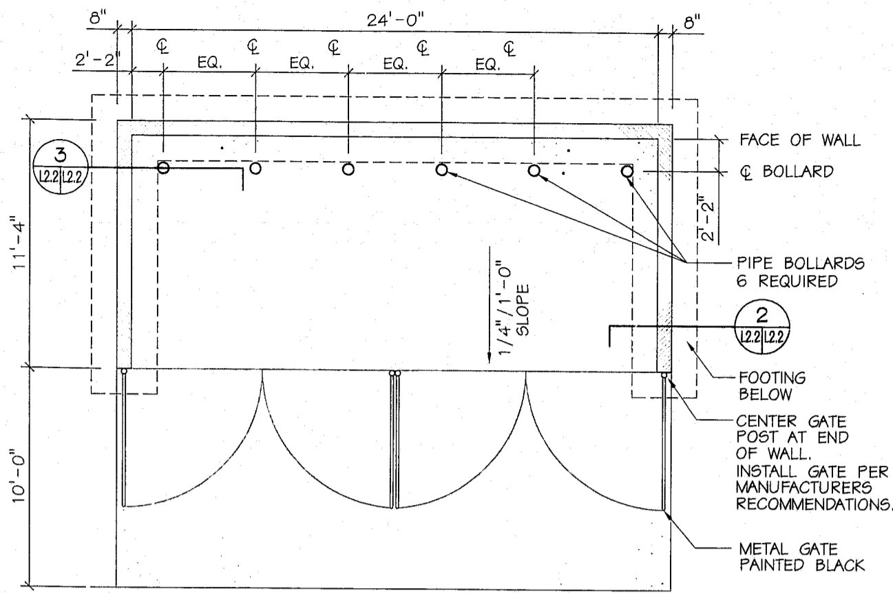
1 TRASH ENCLOSURE PLAN SCALE: 1/4" = 1'-0"
