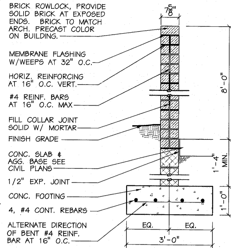
2 TRASH ENCLOSURE SECTION SCALE: 3/4" = 1'-0"
