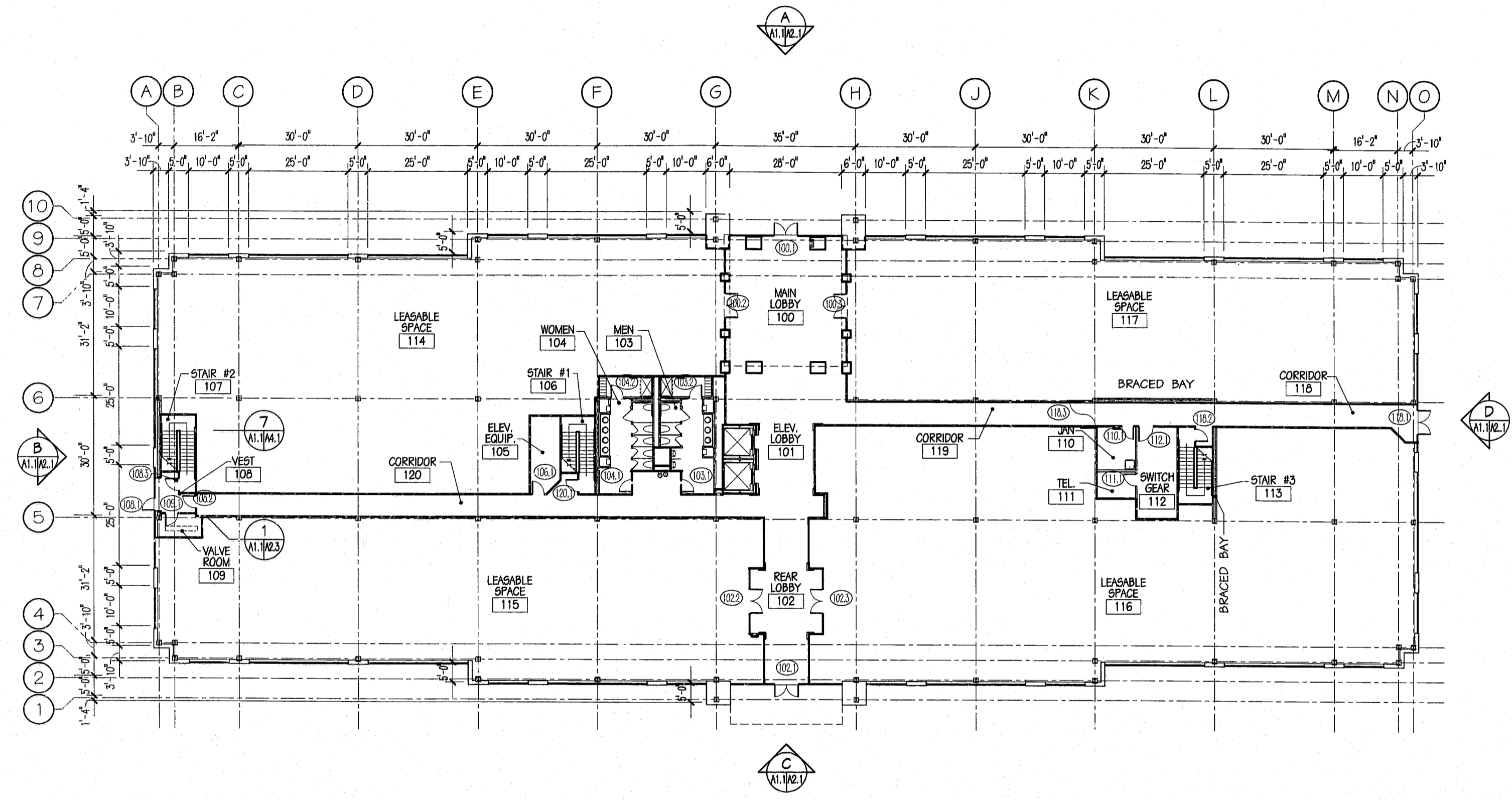
FIRST FLOOR PLAN SCALE: 1/16" = 1'-0"
