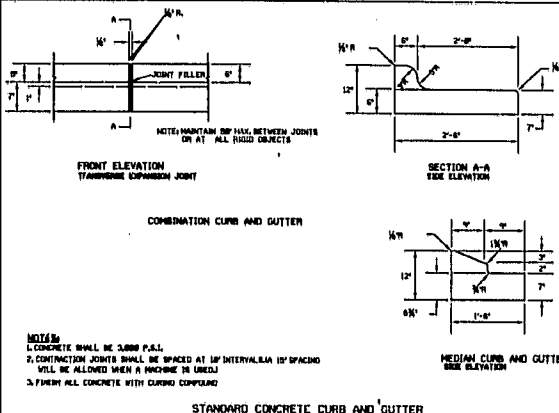
A.B.C. UNDER 2" CURB & GUTTER
