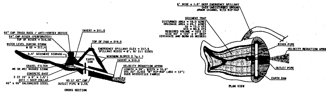
RISER-BARREL SEDIMENT BASIN SEE SHEET C5.0 FOR LOCATION
