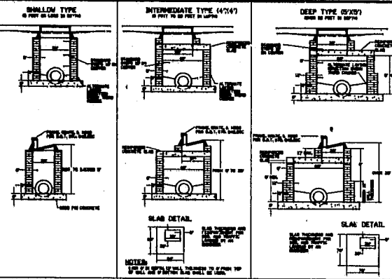
CONCRETE BLOCK OR BRICK CATCH BASIN
