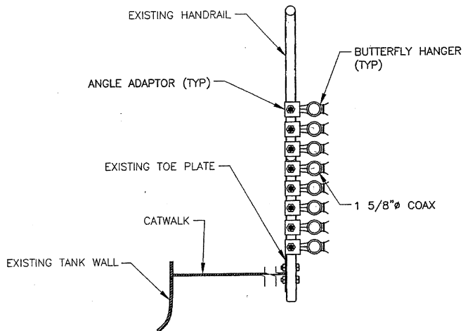
COAX ROUTING AROUND CATWALK DETAIL NOT TO SCALE
