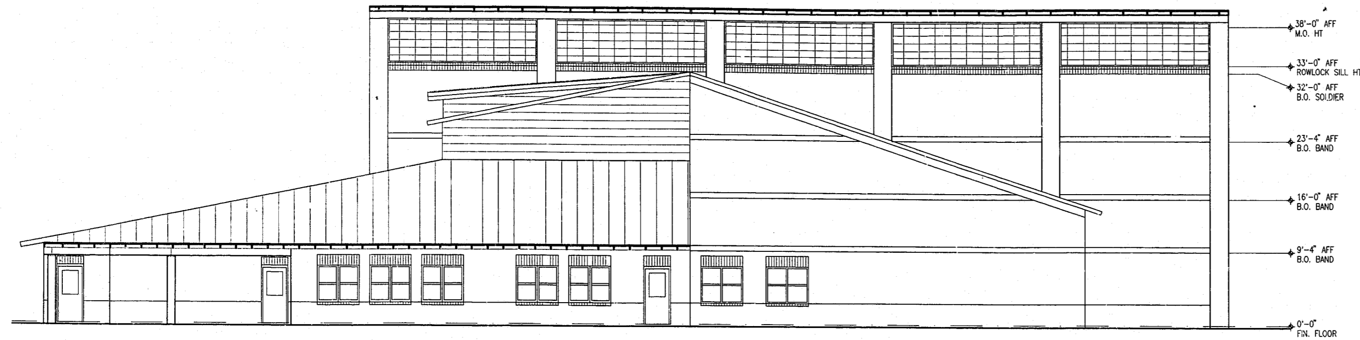
1 EAST SIDE ELEVATION A-5.2 1/8" = 1'-0"
