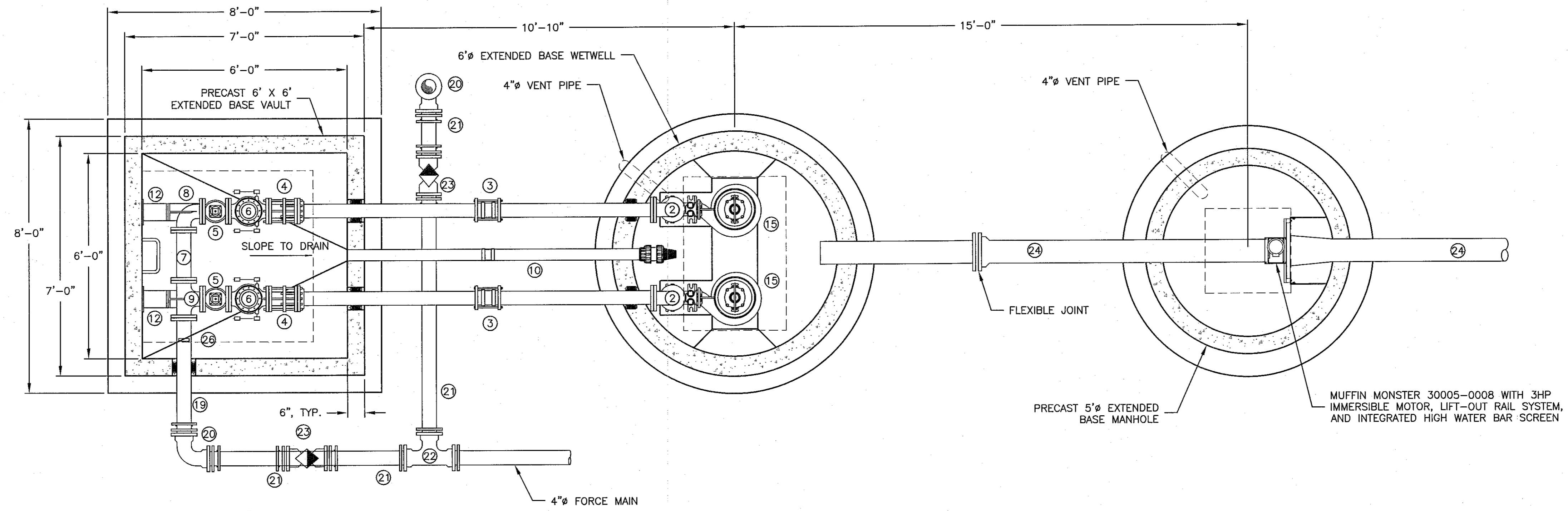
PUMP STATION SITE PLAN 1/2" = 1'-0"
