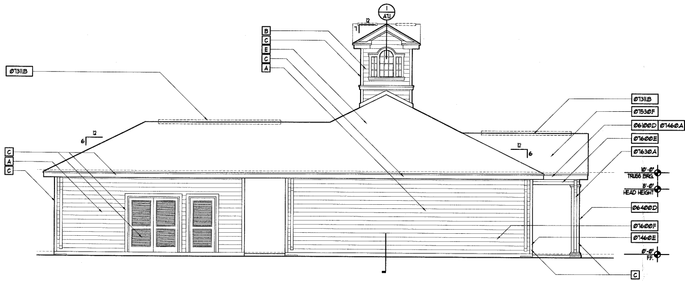
1 LEFT SIDE ELEVATION SCALE: 1/4" = 1'-0"
