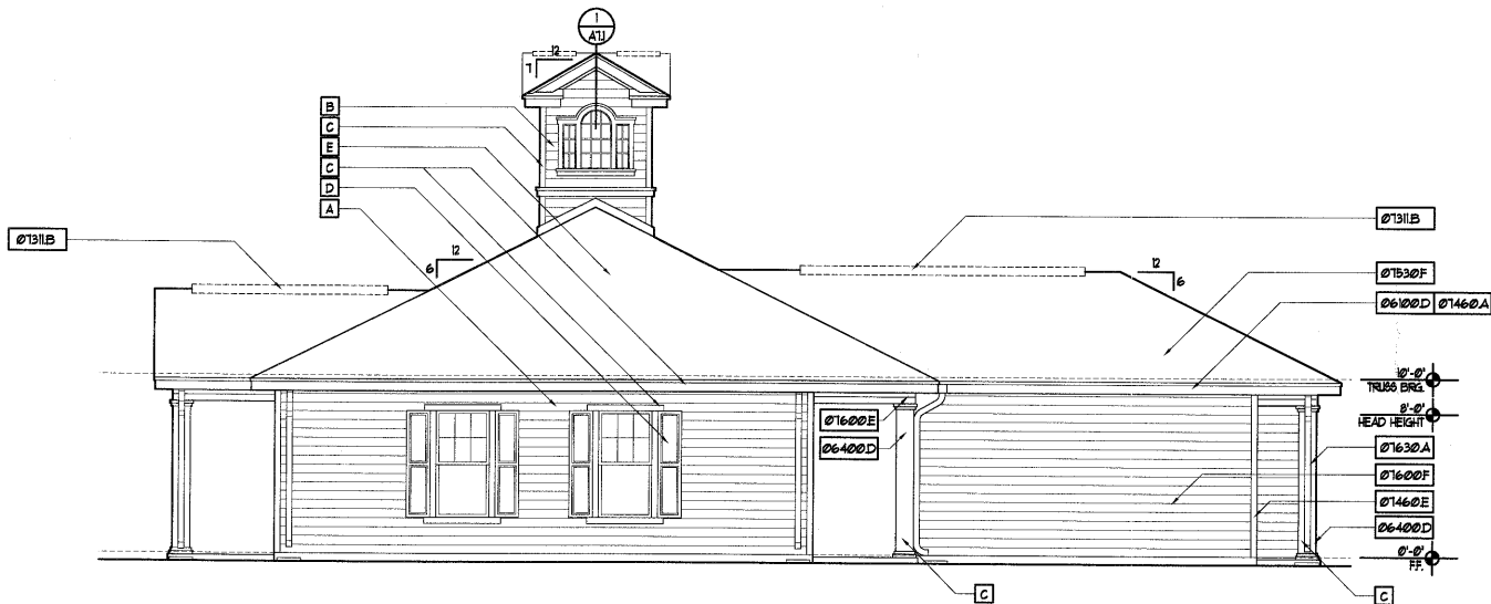
2 RIGHT SIDE ELEVATION SCALE: 1/4" = 1'-0"
