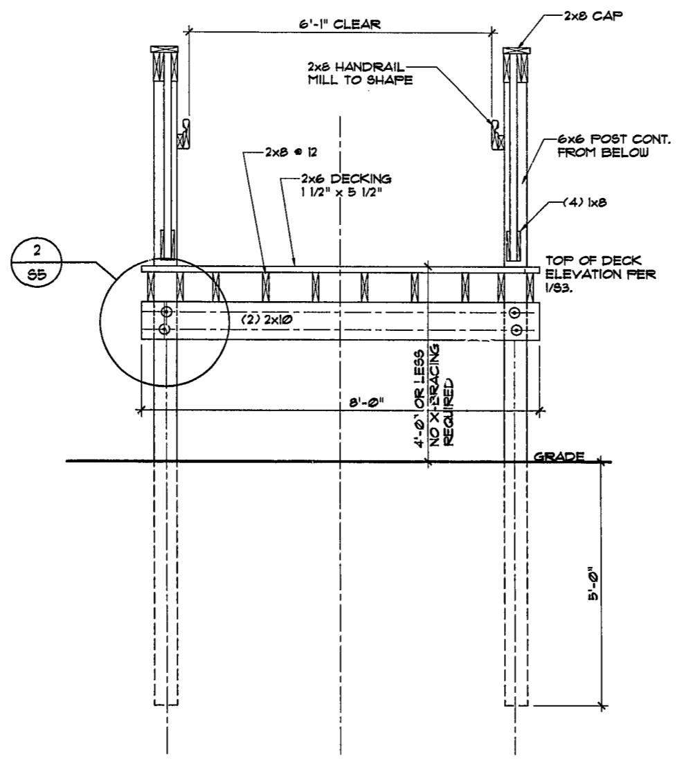
1 SECTION @ BENT S4 SCALE 3/4"=1'-0"
