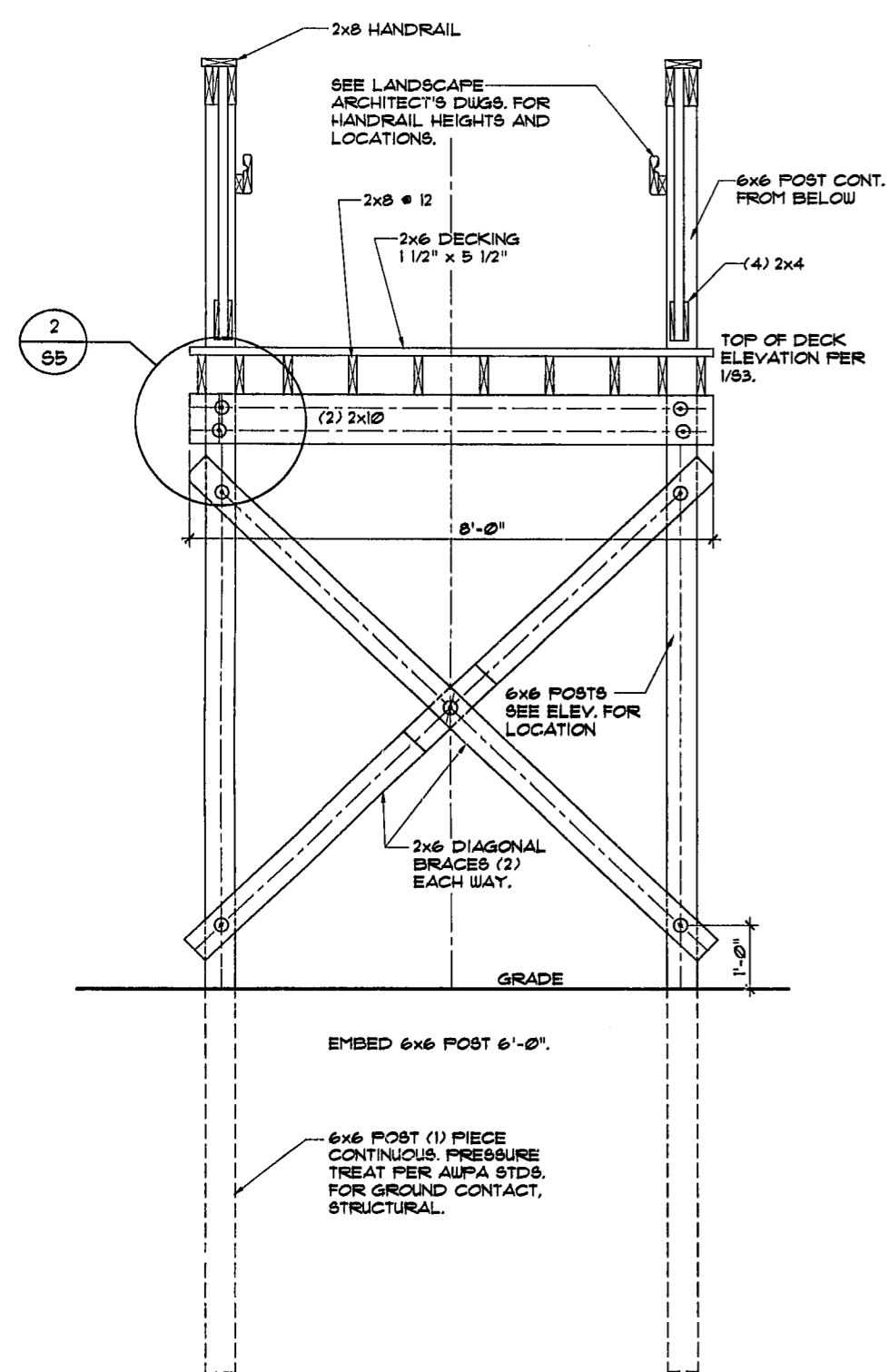
3 SECTION @ BENT S4 SCALE 3/4"=1'-0"
