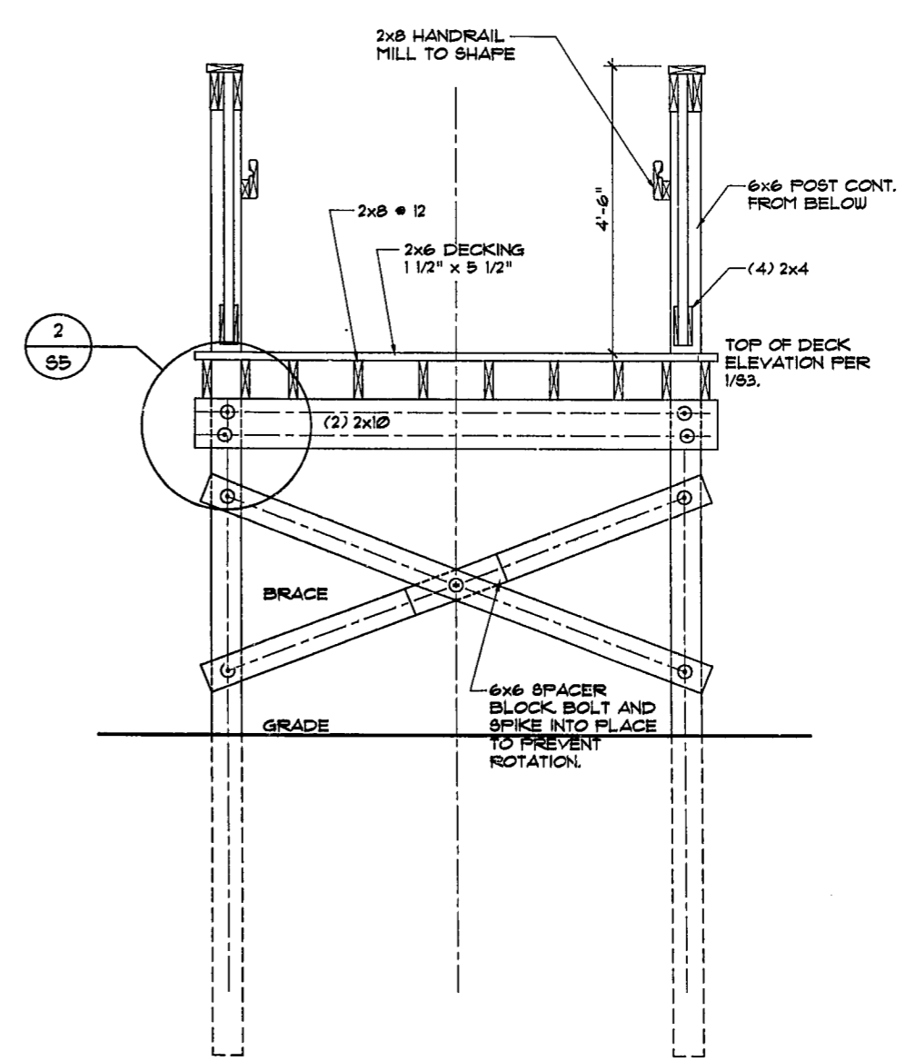
2 SECTION @ BENT S4 SCALE 3/4"=1'-0"
