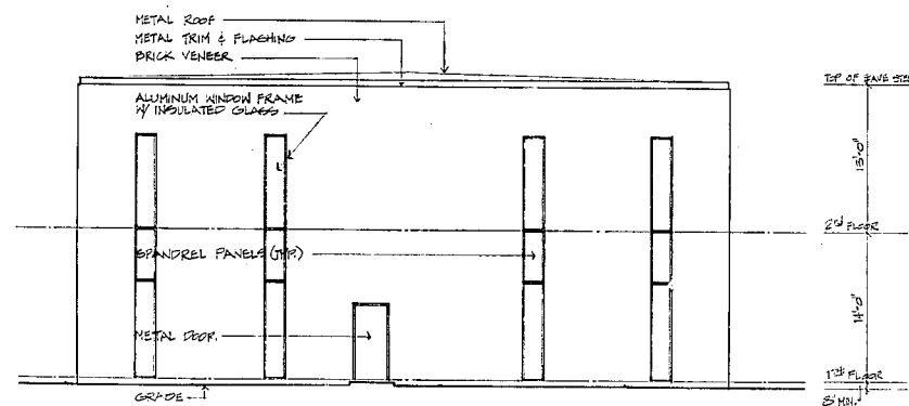
3 LEFT SIDE ELEVATION A-2 1/8" = 1'-0"
