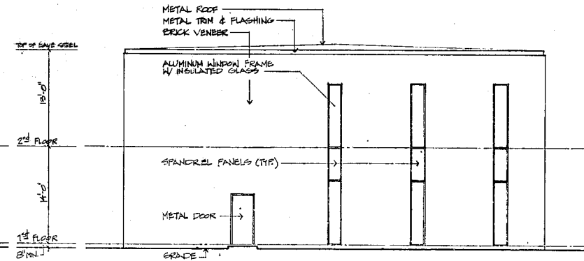
2 RIGHT SIDE ELEVATION A-2 1/8" = 1'-0"
