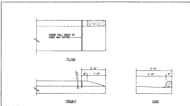
STANDARD METHOD OF ENDING CURB AND GUTTER
