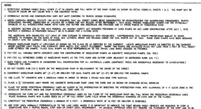
STANDARD WHEELCHAIR RAMP
