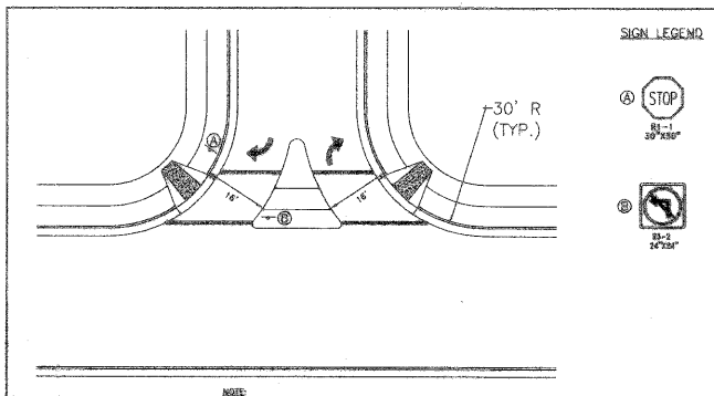
STANDARD RIGHT IN/RIGHT OUT CHANNELIZATION (LIMITED FRONTAGE)
