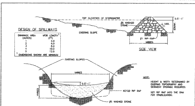
STANDARD GRAVEL & RIP RAP FILTER BASIN
