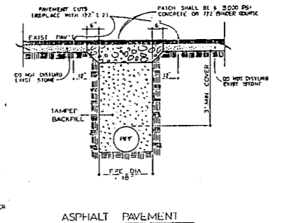
10 TRENCH & PAVEMENT REPAIR SECTIONS 12 N.T.S.
