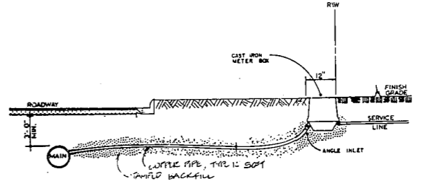
8 3/4" & 1" METER BOX INSTALLATION 12 N.T.S.
