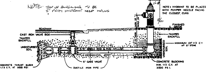
4 HYDRANT INSTALLATION 12 N.T.S.
