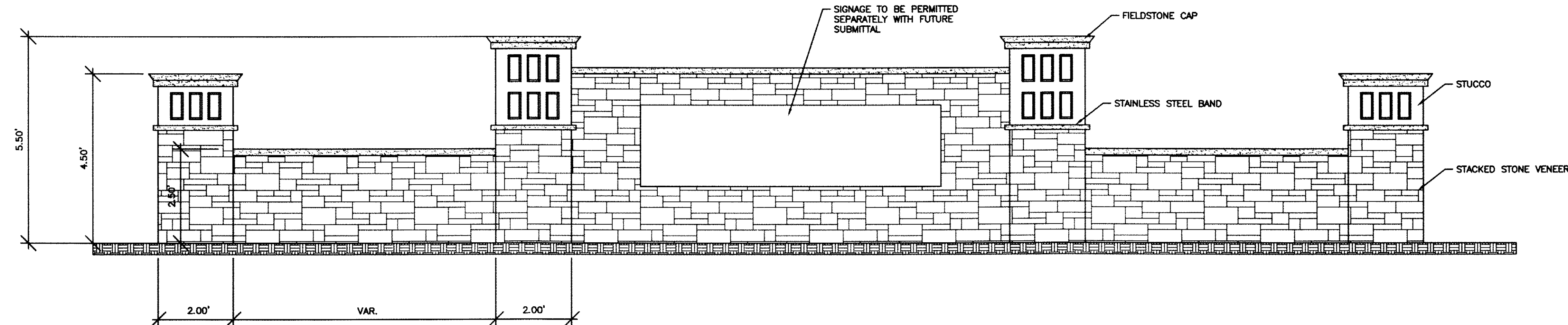
ENTRANCE AND MONUMENTATION ELEVATION
