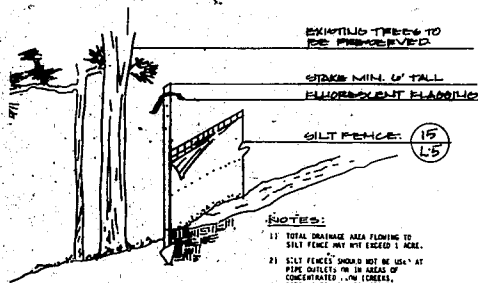
3 TREE PROTECTION FENCE L-5 NOT TO SCALE
