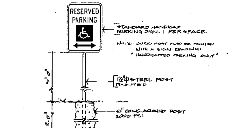
16 HANDICAP PARKING SIGN L-5 NOT TO SCALE
