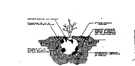
18 SHRUB PLANTING L-5 NOT TO SCALE
