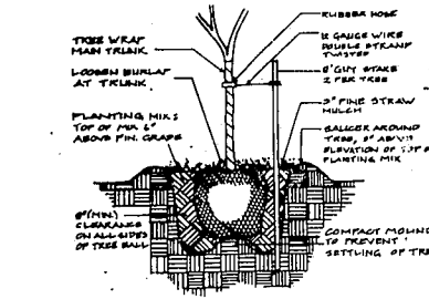
20 0-3" CALIPER TREE L-5 NOT TO SCALE
