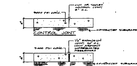
17 CONCRETE SIDEWALK & JOINT L-5 NOT TO SCALE
