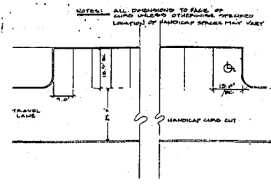
10 TYPICAL PARKING SPACES L-5 NOT TO SCALE
