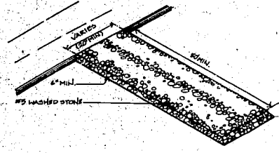
1 CONSTRUCTION ENTRANCE L-5 NOT TO SCALE
