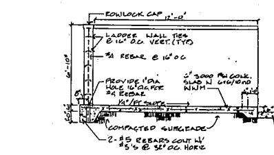
13 DUMPSTER SCREEN WALL L-5 NOT TO SCALE
