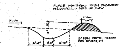
2 TEMPORARY DIVERSION L-5 NOT TO SCALE
