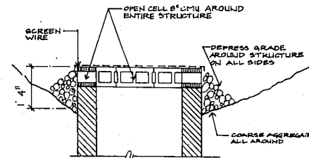
7 PROTECTED DRAINAGE STRUCTURE L-5 NOT TO SCALE
