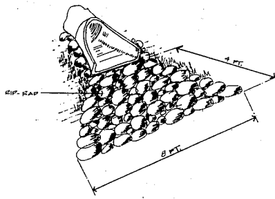
11 FLARED END SECTION L-5 NOT TO SCALE
