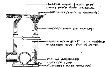
6 JUNCTION BOX L-5 NOT TO SCALE
