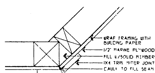
CUPOLA DETAIL
