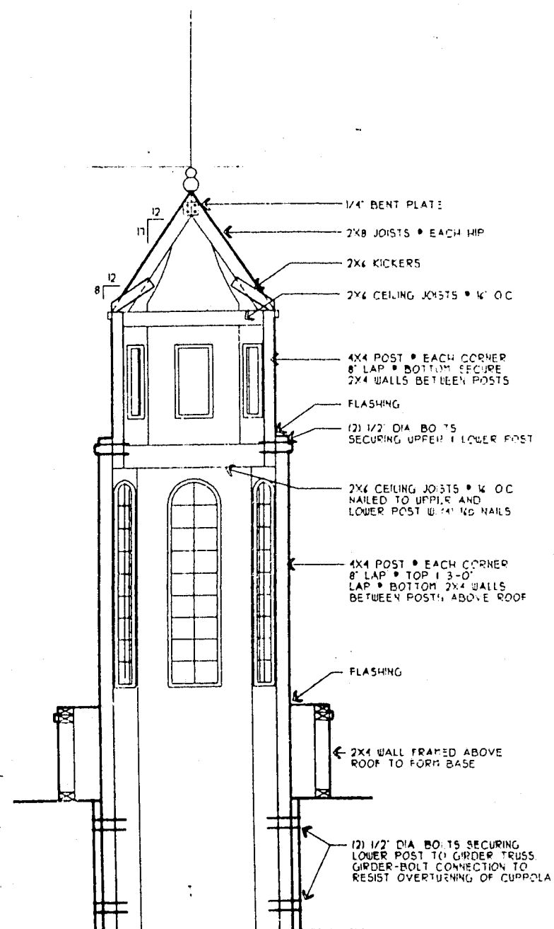
CUPOLA SECTION
