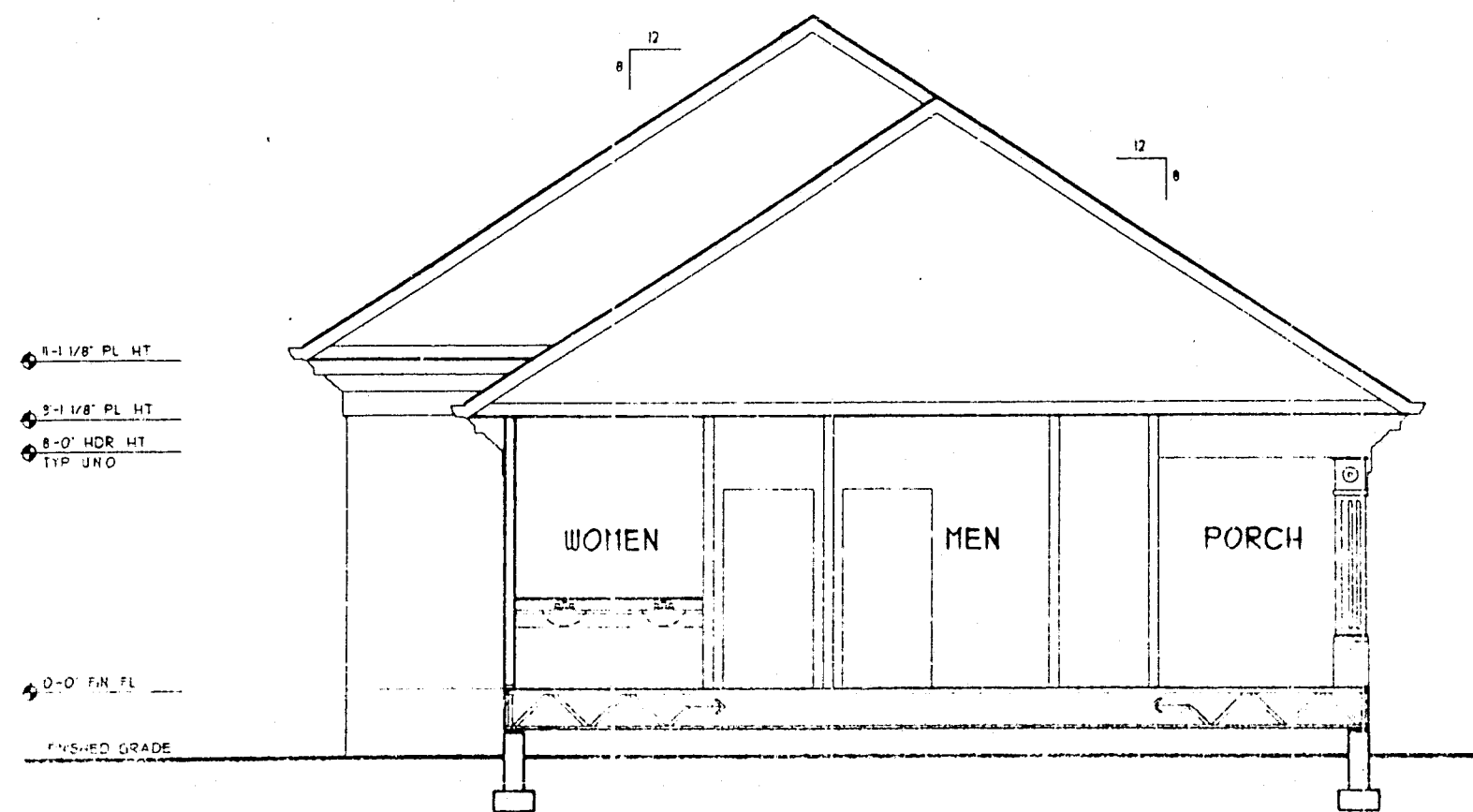
SECTION C-C LOOKING SOUTHEAST
