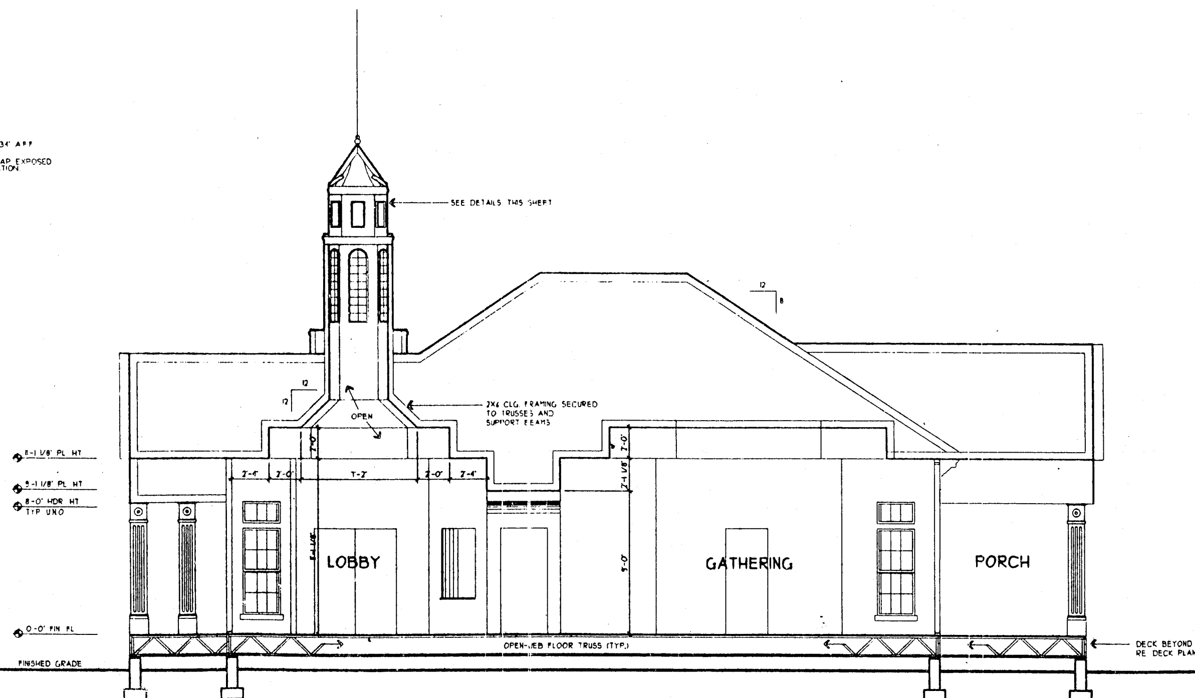
SECTION B-B LOOKING SOUTHEAST
