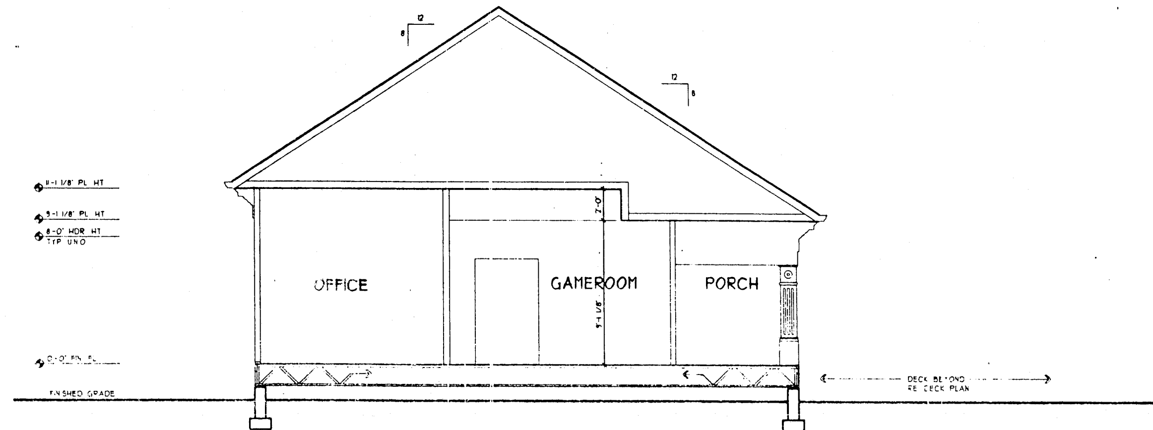
SECTION A-A LOOKING SOUTHEAST
