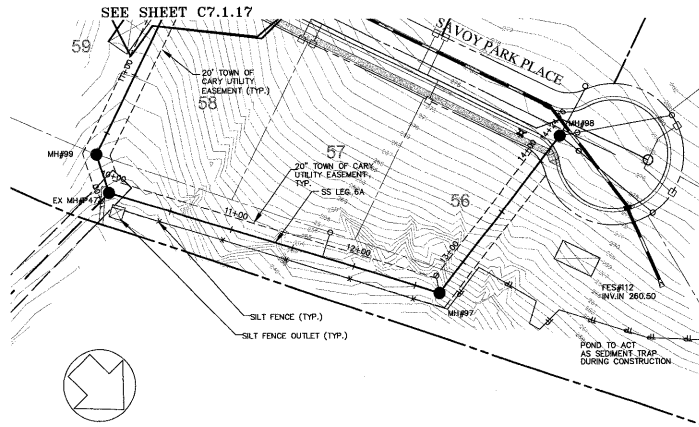
LEG 6A PLAN VIEW
