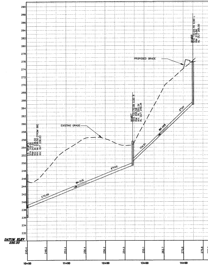
LEG 6A PROFILE
