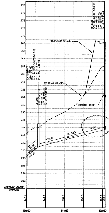
LEG 6B PROFILE
