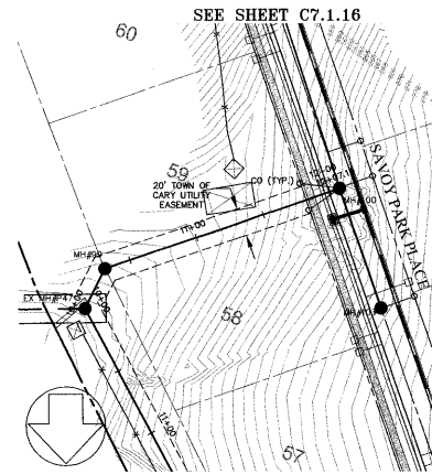
LEG 6B PLAN VIEW
