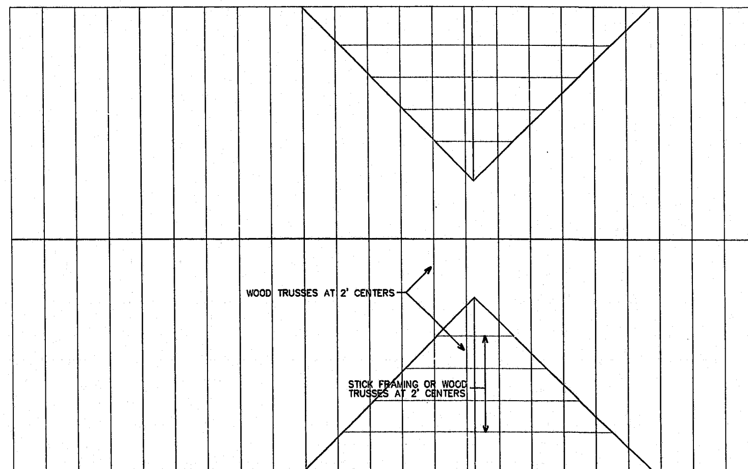
02 FRAMING PLAN A4.01 SCALE: 1/4" = 1'-0"
