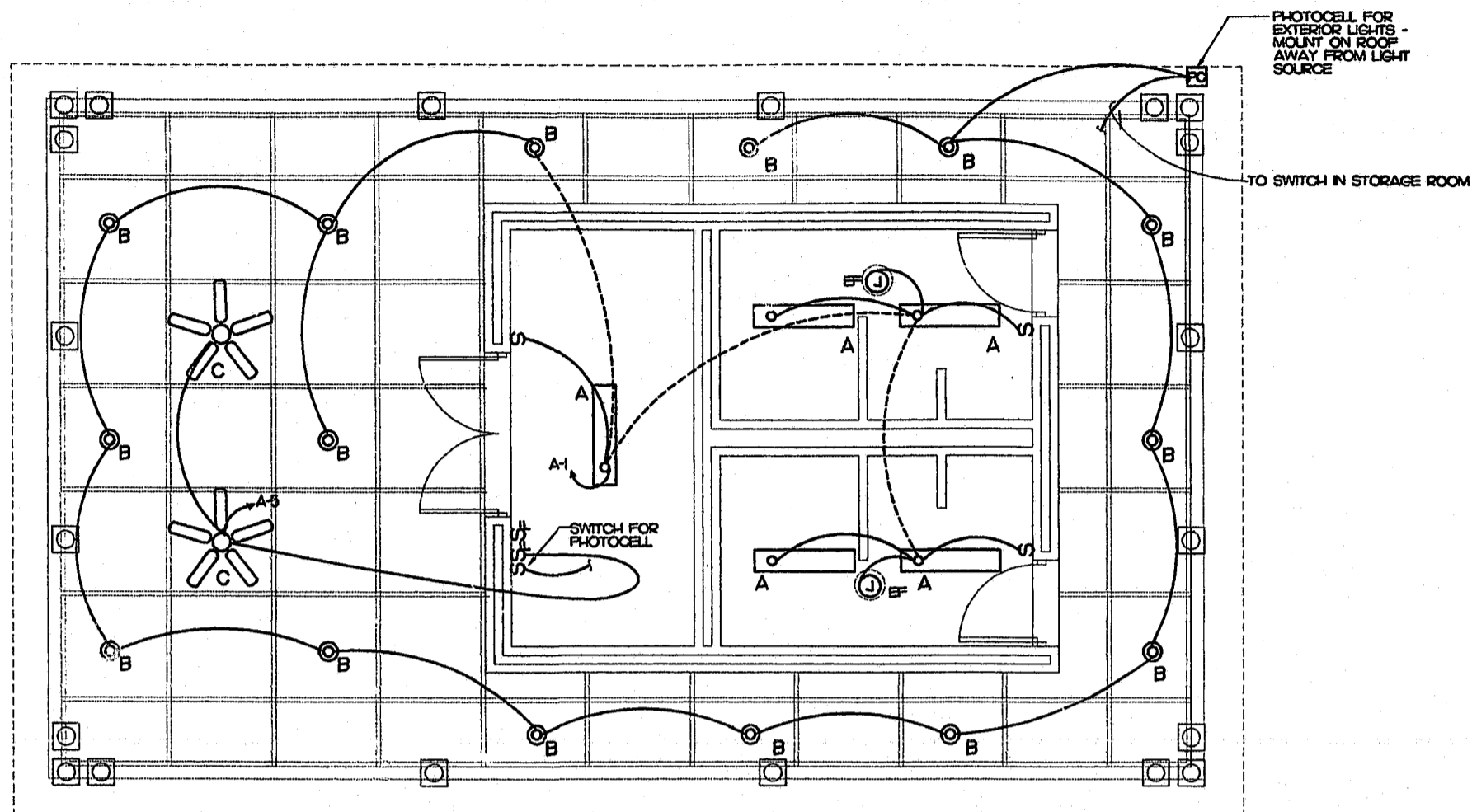
01 LIGHTING PLAN E.01 SCALE: 1/4" = 1'-0"
