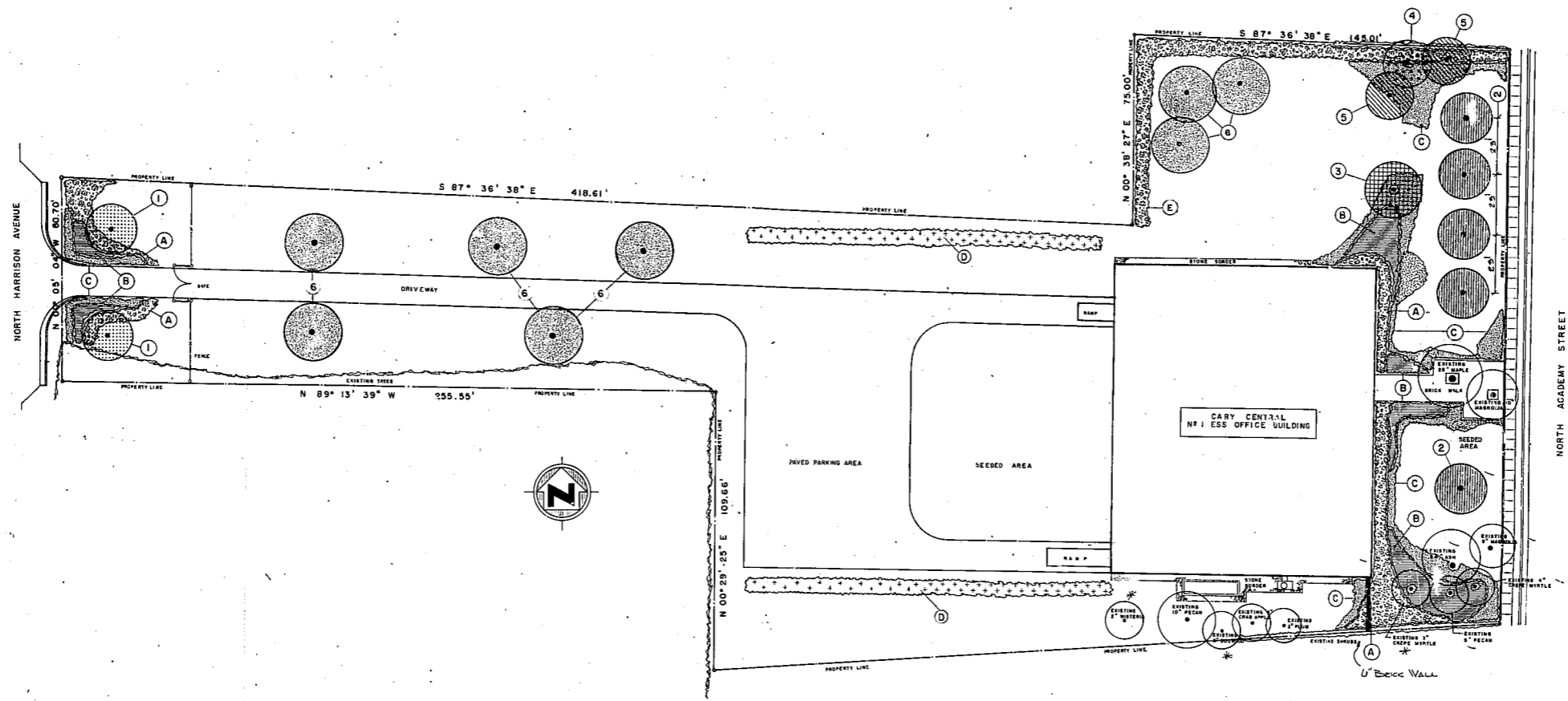
LANDSCAPING SITE PLAN 1" = 20'
