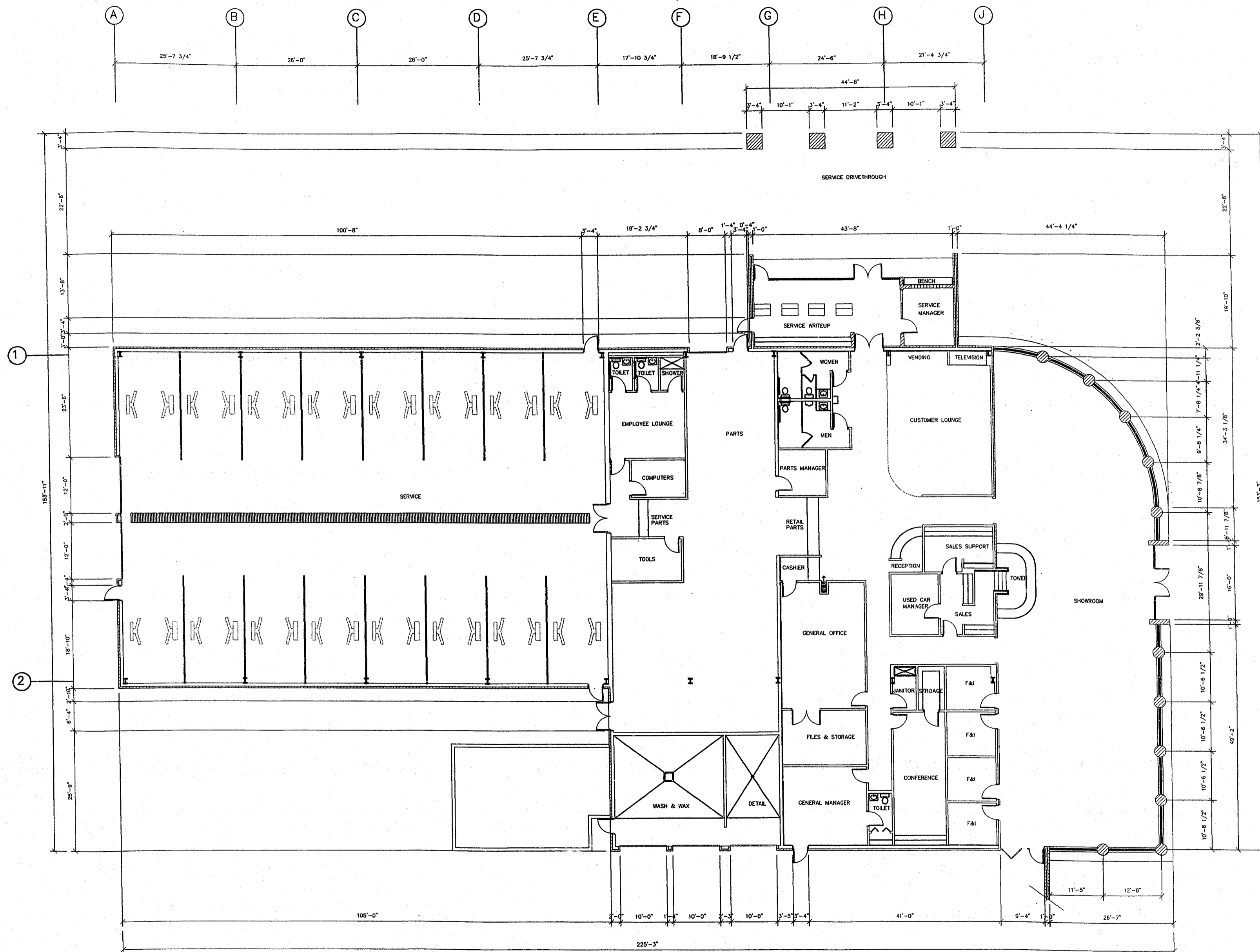
FLOOR PLAN 3/16"=1'-0"
