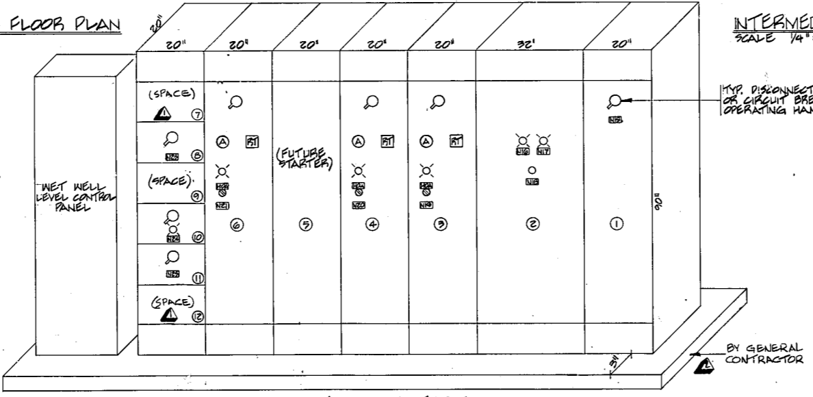
MOTOR CONTROL CENTER "MCC1" SCALE 3/4" = 1'-0"
