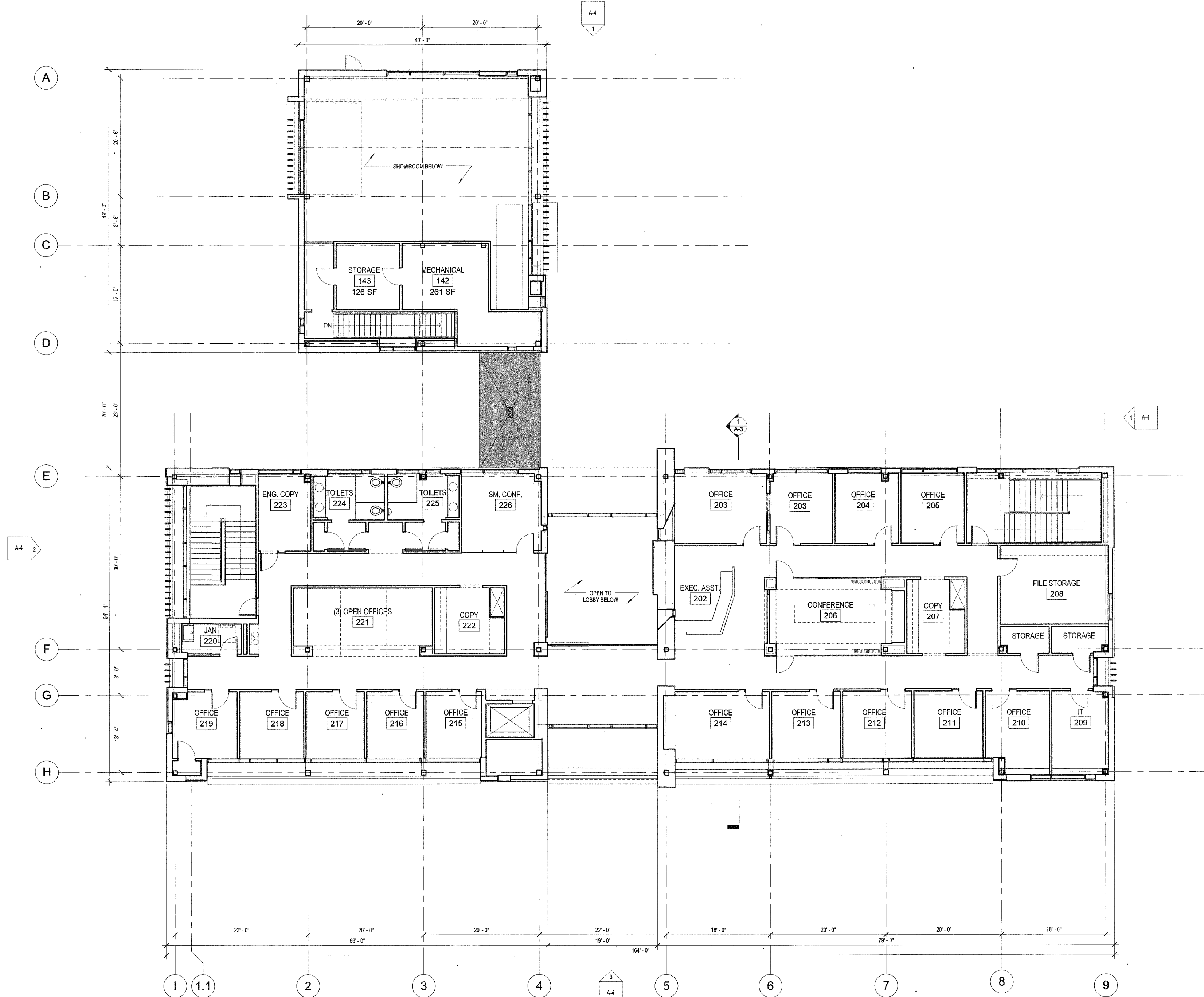
1 SECOND FLOOR PLAN A-2
