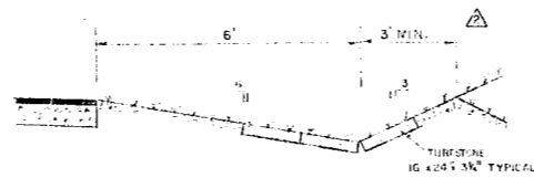
SECTION TYPICAL TURFSTONED LINED SWALE NOT TO SCALE
