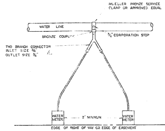
DOUBLE WATER SERVICE NOT TO SCALE
