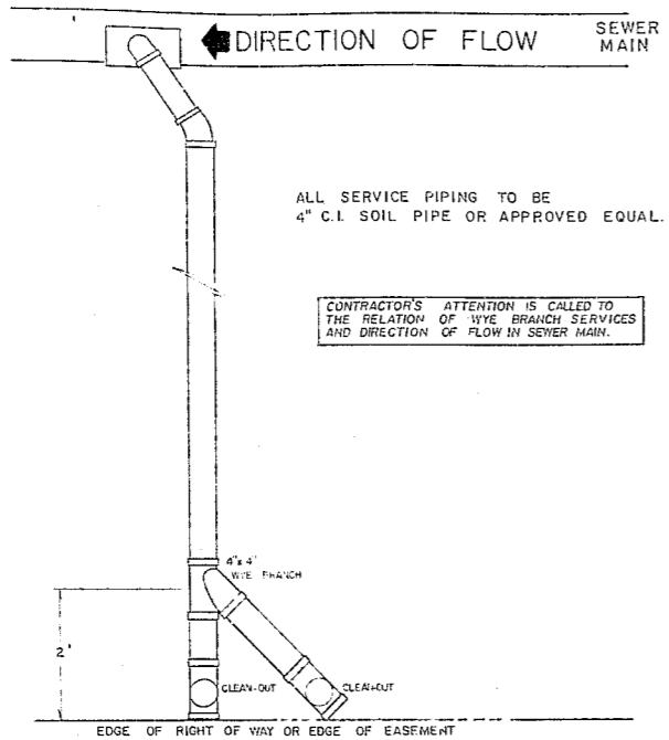
MULTIPLE SANITARY SEWER SERVICES FROM SINGLE SEWER TAP NOT TO SCALE
