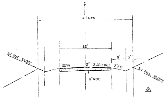
TYPICAL SECTION TWIN OAKS PLACE NOT TO SCALE
