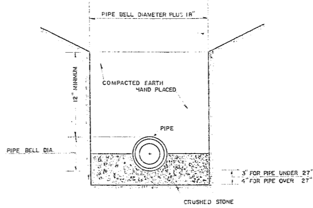
CLASS 'B' BEDDING NOT TO SCALE
