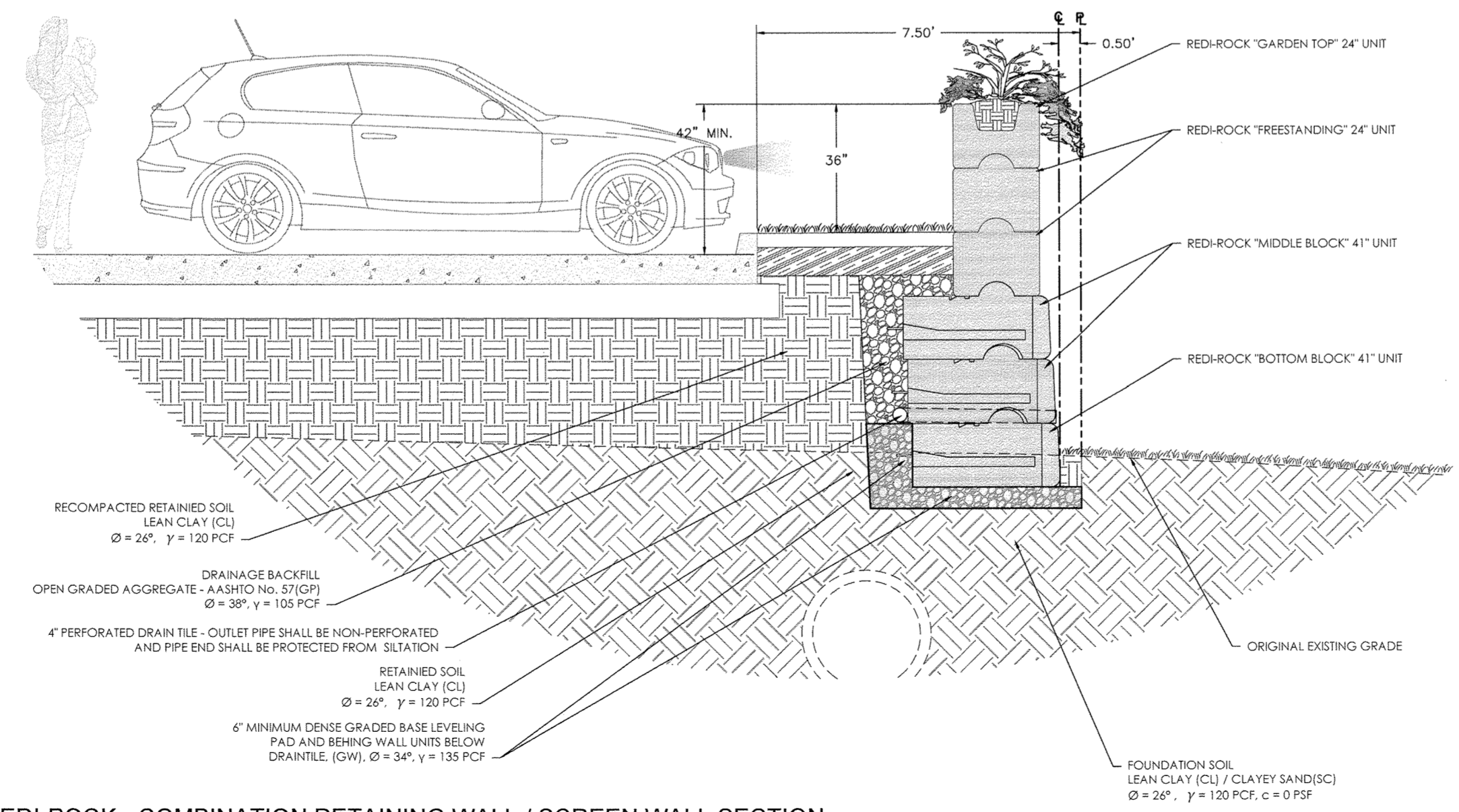
REDI-ROCK - COMBINATION RETAINING WALL / SCREEN WALL SECTION
