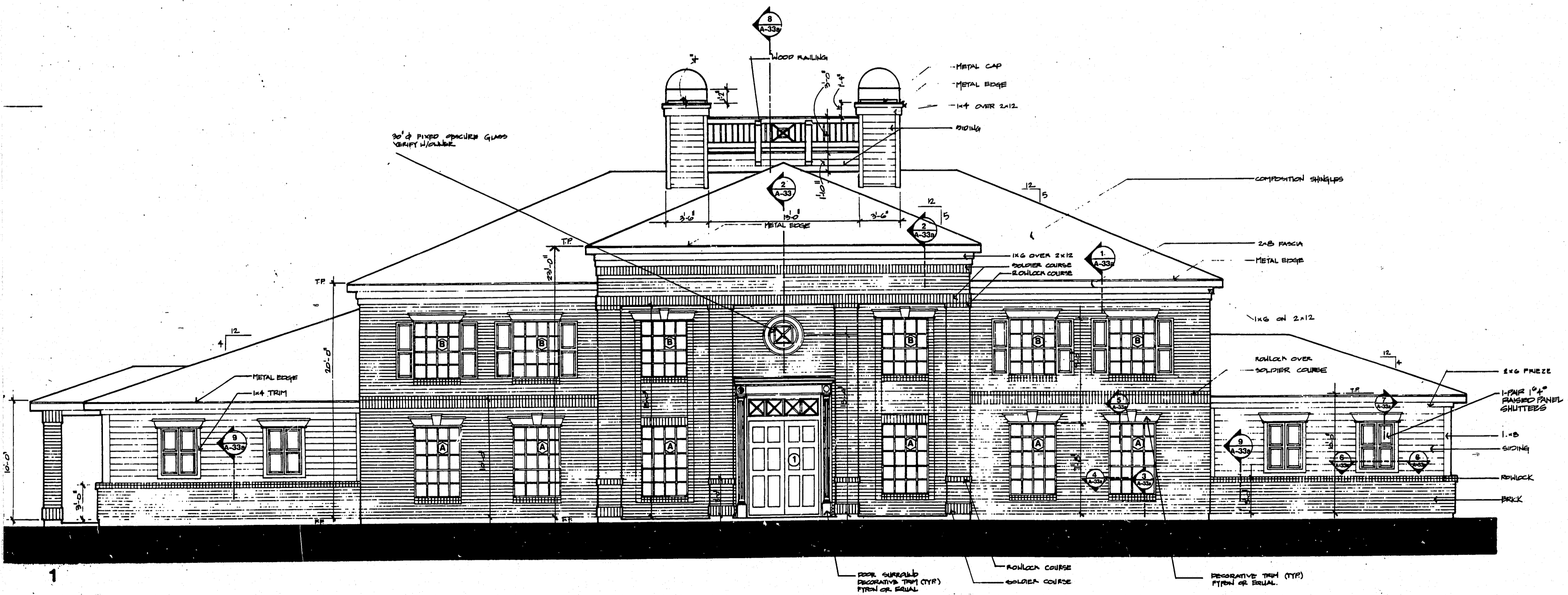
OFFICE/CLUB ELEVATION SCALE: 1/4" = 1'-0"
