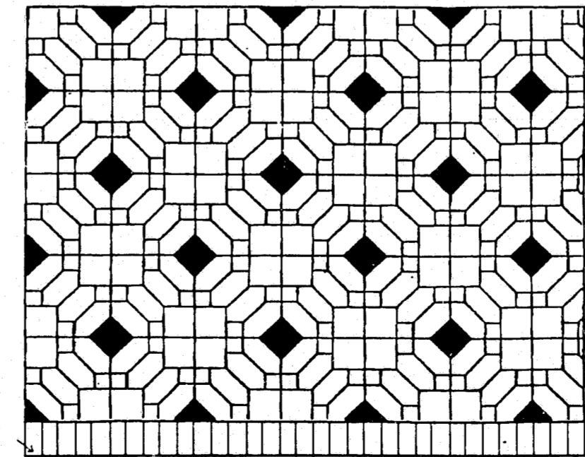
TYPICAL PAVER LAYOUT
