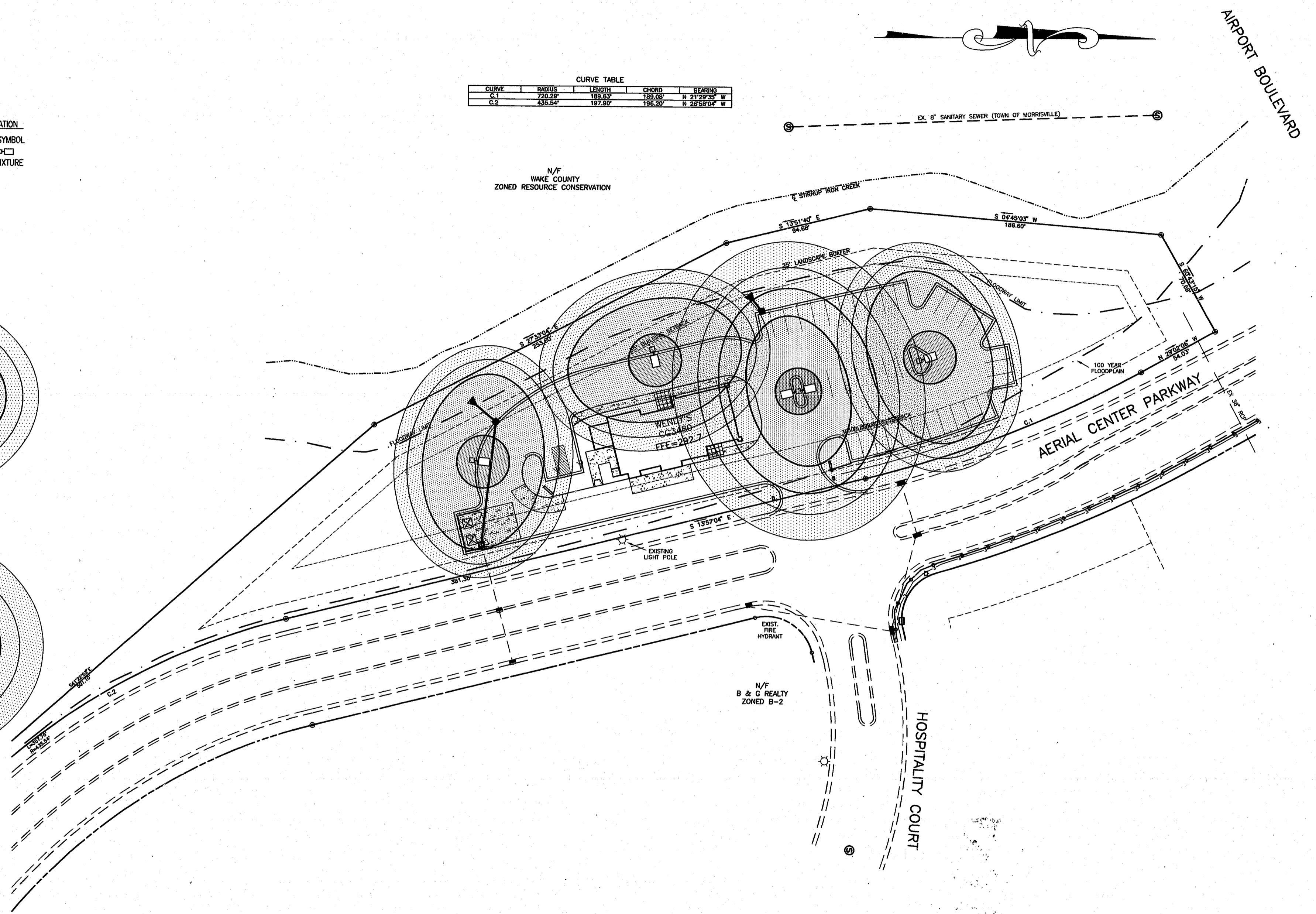
TYPICAL FOOTCANDLES
