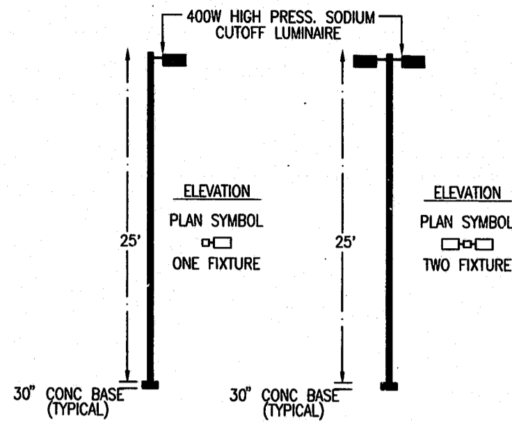
LIGHTING LEGEND
