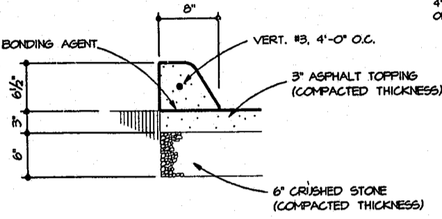
EXTRUDED CURB DETAIL
