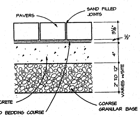
PAVER DETAIL
