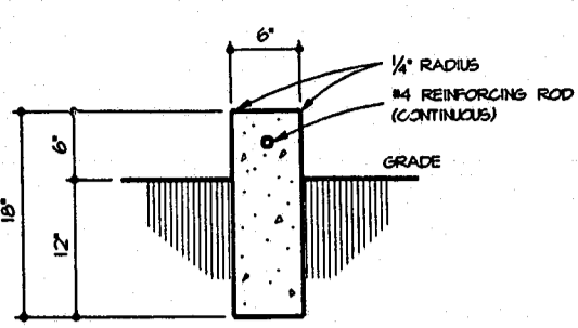
CONCRETE CURB DETAIL
