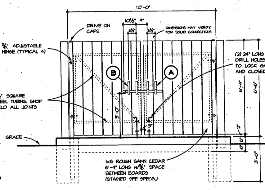
TYPICAL FRONT ELEVATION
