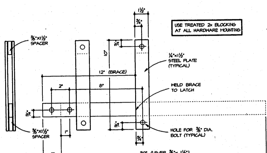
GATE LATCH DETAIL "B"
