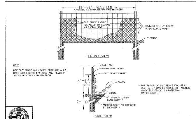
STANDARD TEMPORARY SILT FENCE DETAIL No. 04000.01 SHEET 1 OF 1
