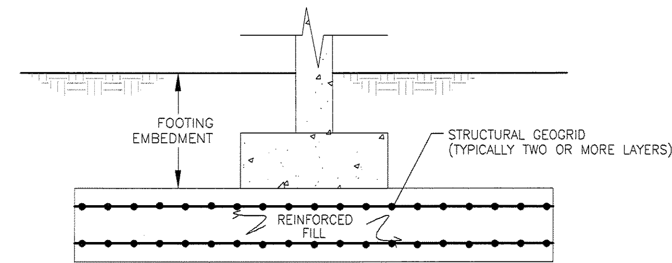
TYPICAL FOOTING CROSS-SECTION NOT TO SCALE
