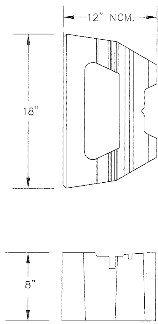
MESA STANDARD UNIT NOT TO SCALE
