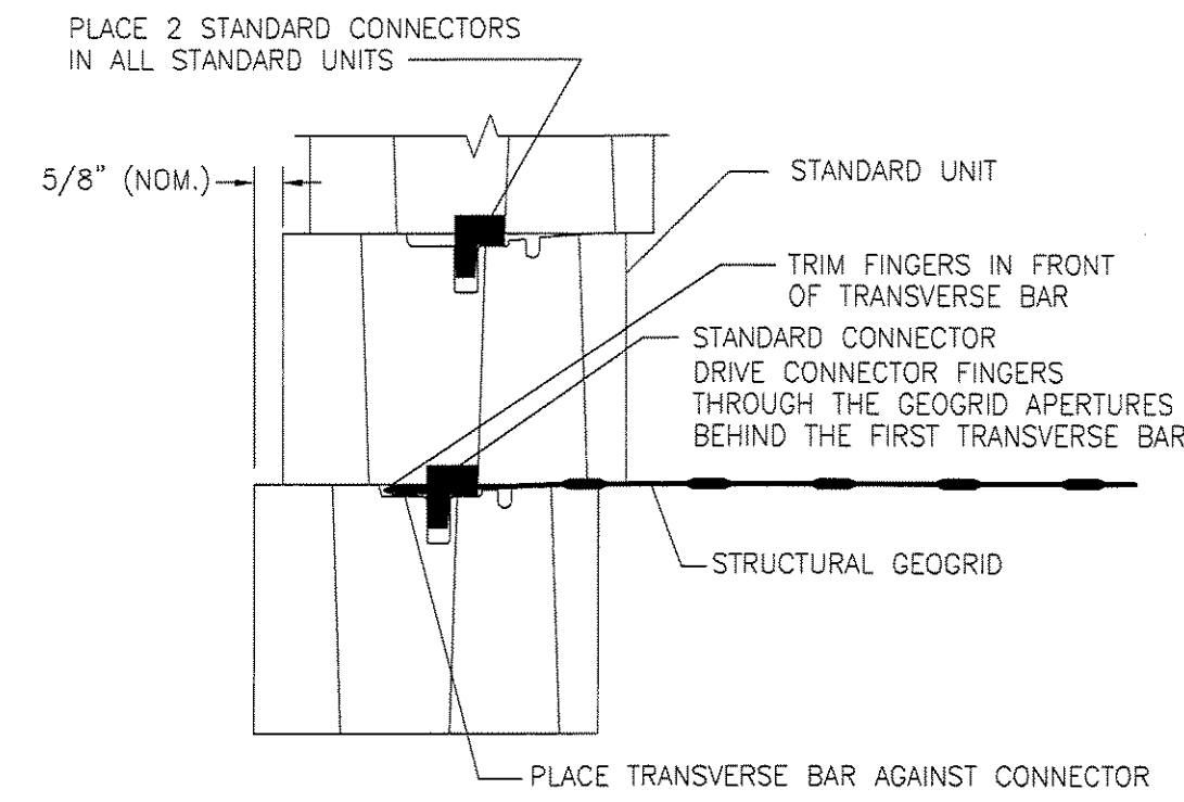
MESA STANDARD UNIT AND GEOGRID CONNECTION DETAIL NOT TO SCALE
