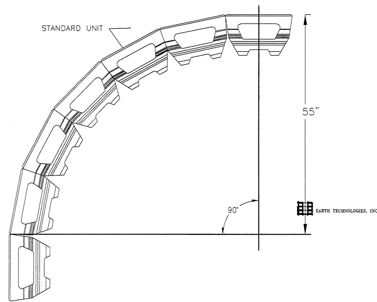
90° CURVE DETAIL STANDARD UNIT NOT TO SCALE
