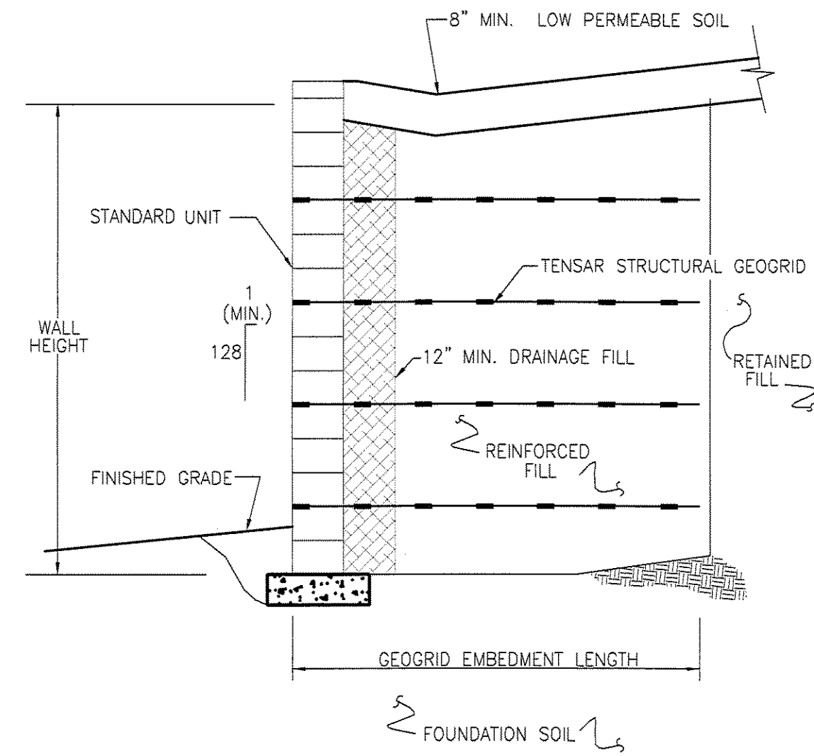
TYPICAL CROSS-SECTION NOT TO SCALE
