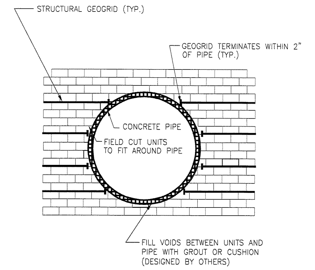
WALL DETAIL AT CONCRETE PIPE OUTLETS NOT TO SCALE
